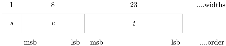
Figure H.1: Single Format. msb means most significant bit , lsb means least significant bit
