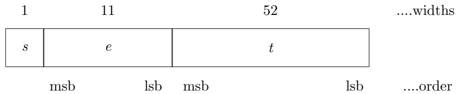
Figure H.2: Double Format. msb means most significant bit , lsb means least significant bit
