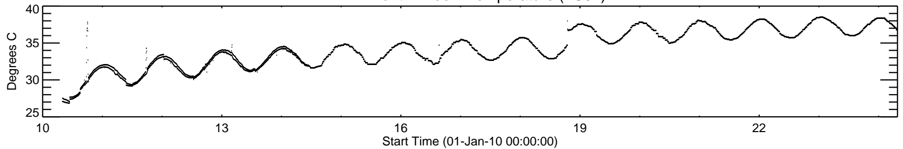
HMI Front Window Temperature (TS01)
