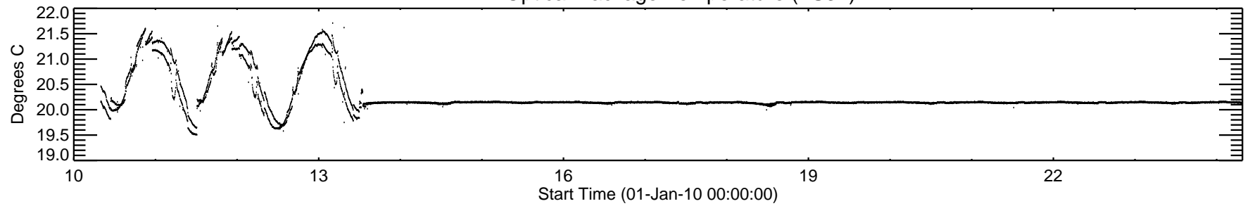
HMI Telescope Tube Temperature (TS06)
