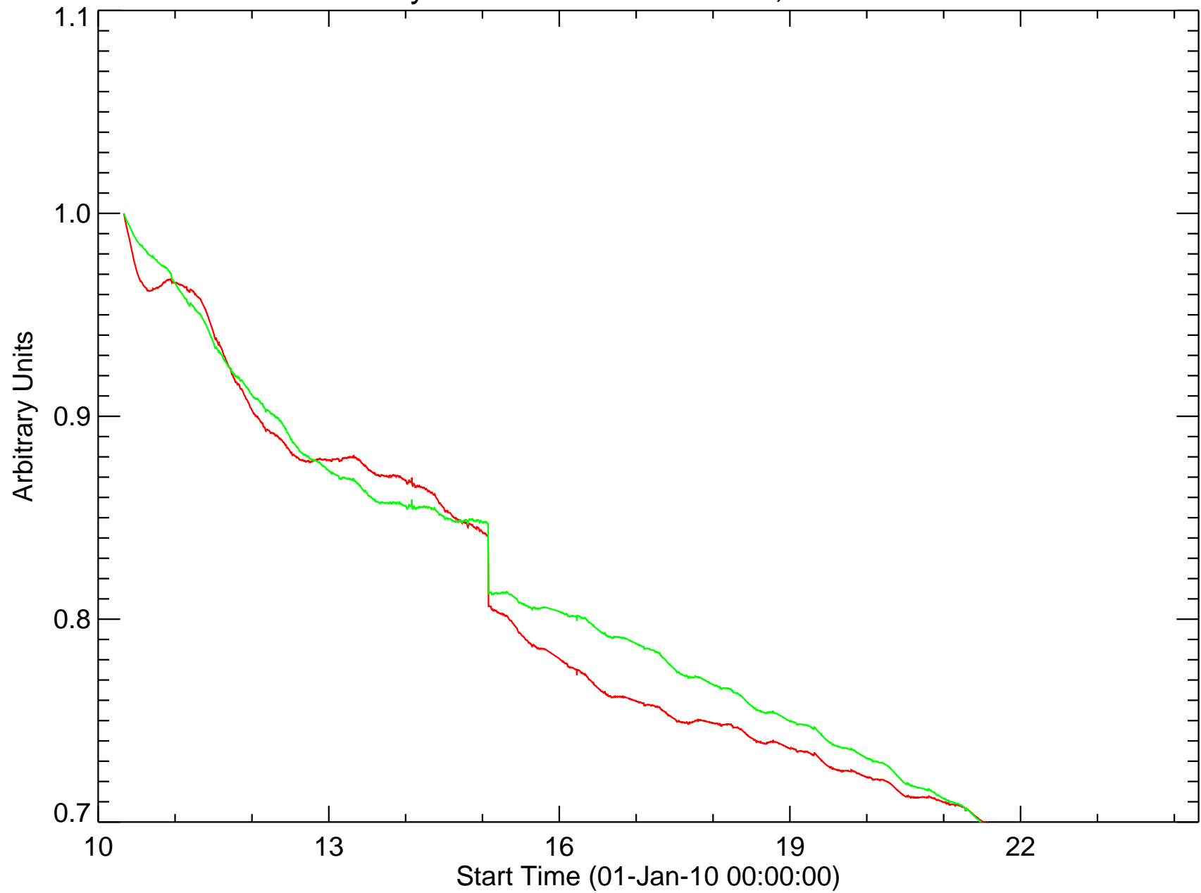
HMI Intensity Corrected for Distance; Normalized Mean
