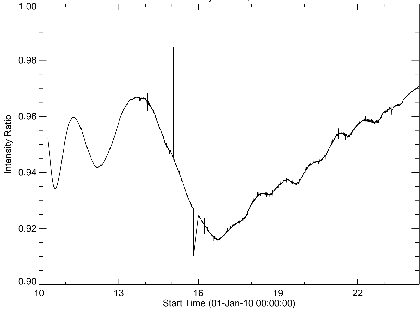
HMI Continuum Intensity Mean; Camera 1 to Camera 2
