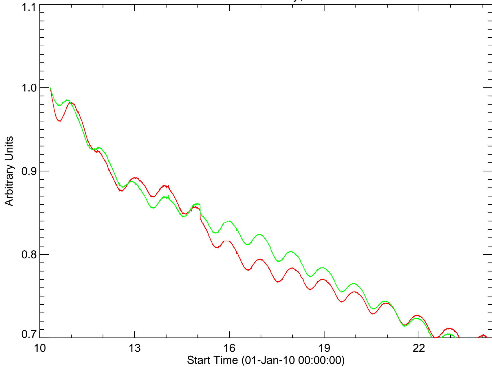
HMI Continuum Tuned Intensity; Normalized Median
