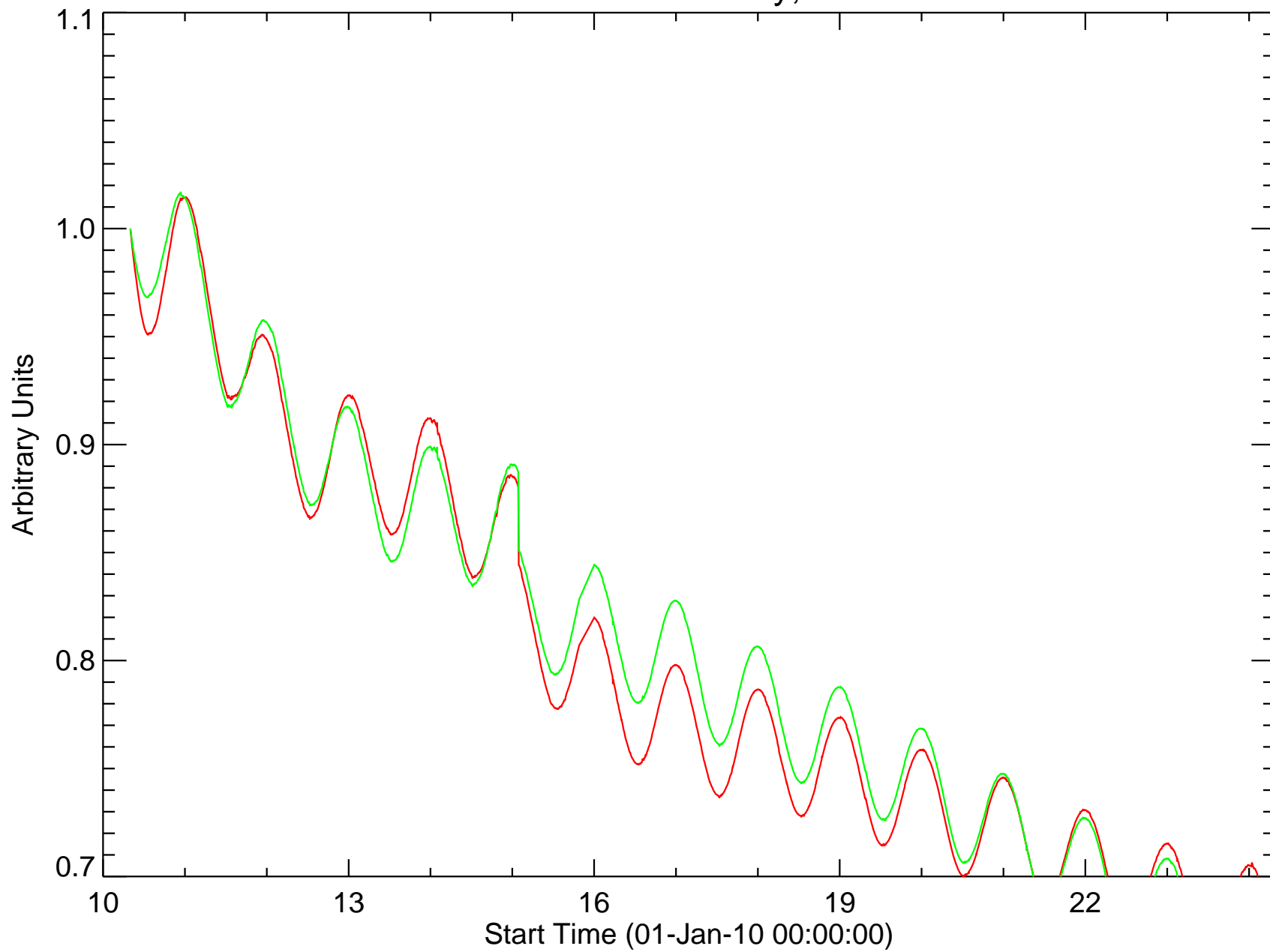
HMI Continuum Tuned Intensity; Normalized Mean
