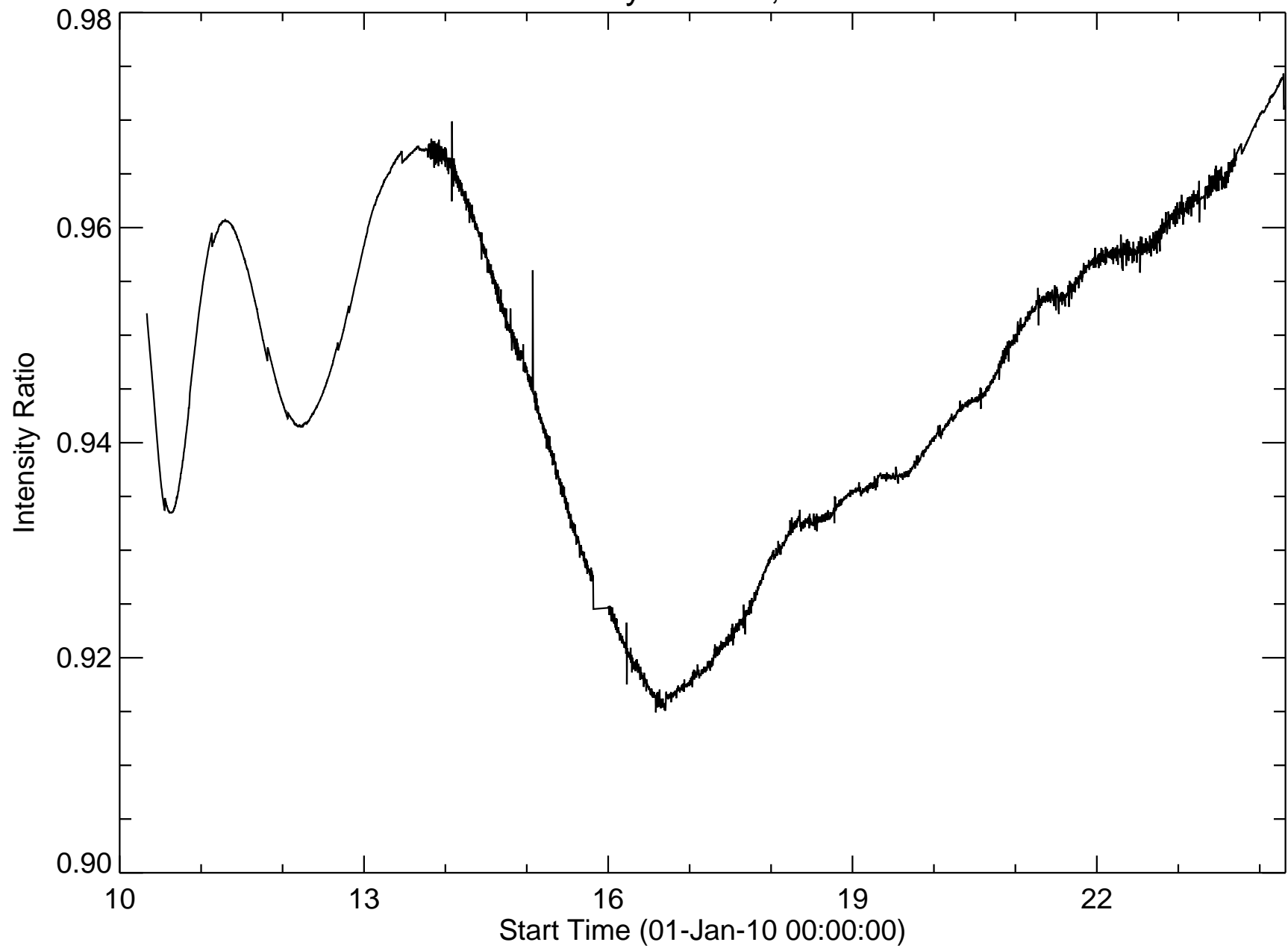
HMI Continuum Intensity Median; Camera 1 to Camera 2
